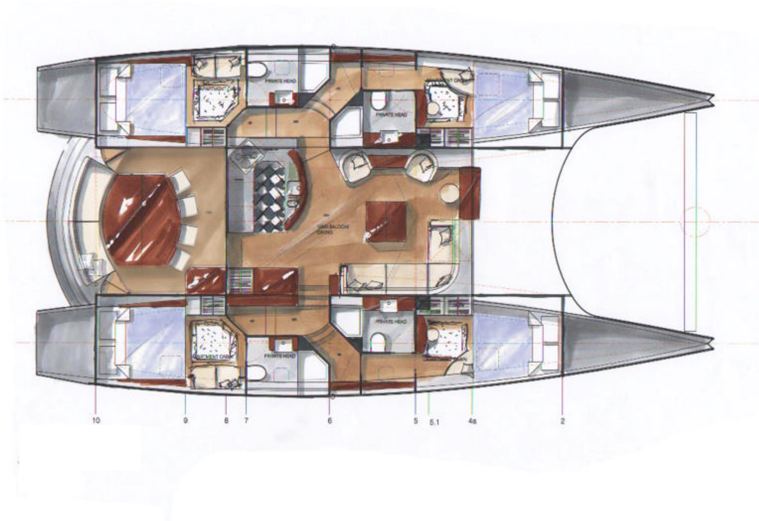
ISARA 50 SAIL 4 CABIN LAYOUT
